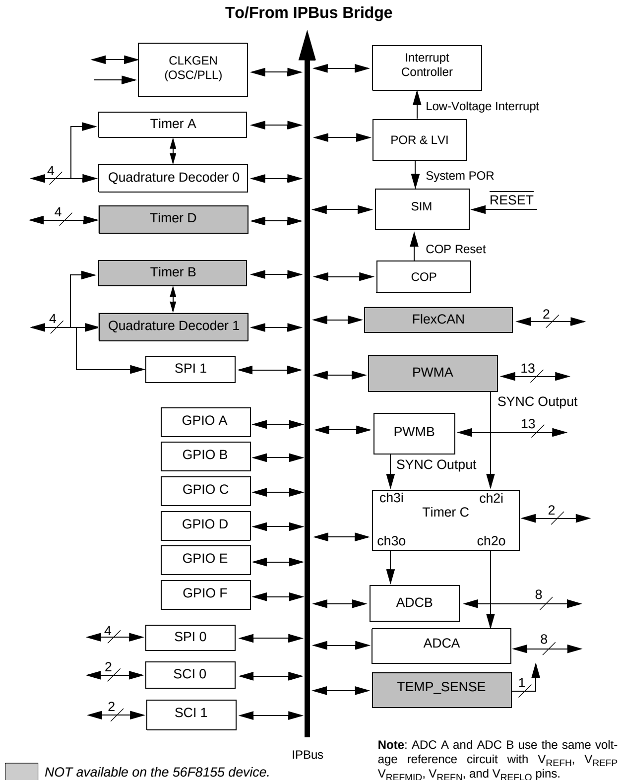
Figure 1-2 Peripheral Subsystem
