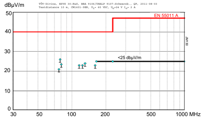
Fig. 14a Typical radiated emissions of CM1601-9ER according to IEC/EN 55011/22, normalized to a distance of 10 m, measured at V_i = 60 VDC and I_{o \text{ nom}} .
