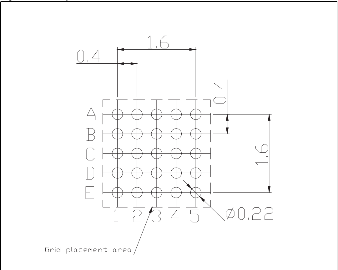
Figure 11. Footprint recommendation
