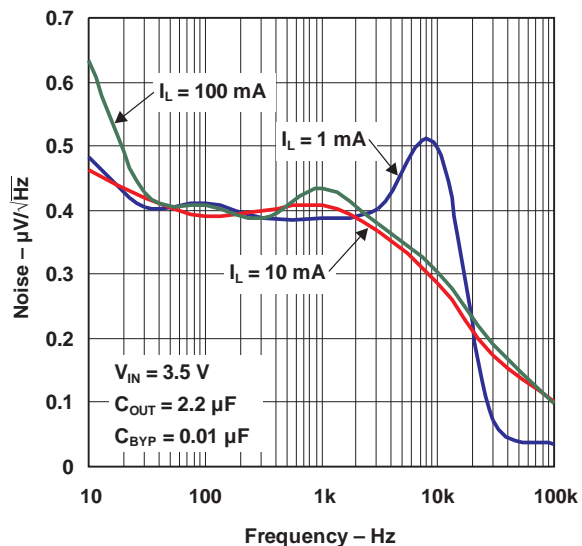
NOISE PERFORMANCE
