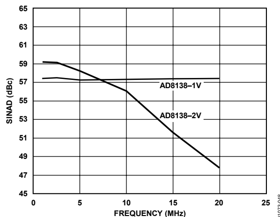
Figure 49. AD9203 SINAD @ -0.5 dBFS AD8138
