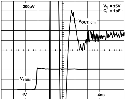
Figure 25. Settling Time
