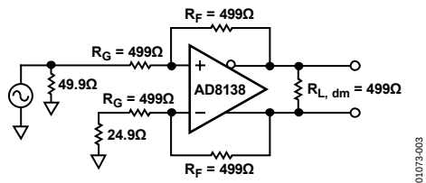
Figure 39. Basic Test Circuit
