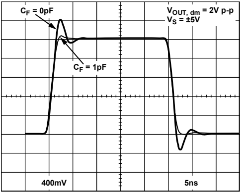
Figure 24. Large Signal Transient Response
