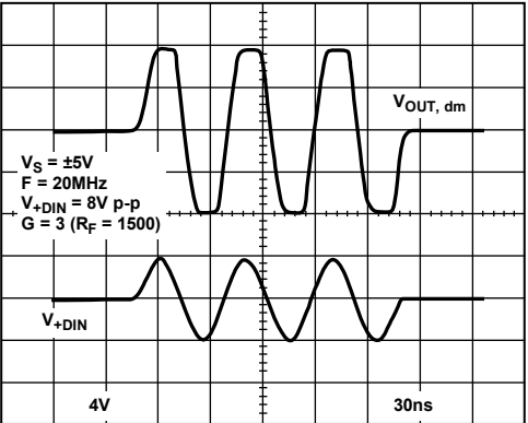
Figure 26. Output Overdrive
