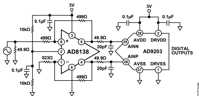
Figure 47. AD8138 Driving an AD9203, a 10-Bit, 40 MSPS A/D Converter
