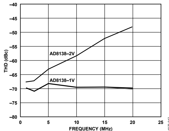
Figure 48. AD9203 THD @ -0.5 dBFS AD8138
