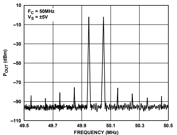
Figure 19. Intermodulation Distortion
