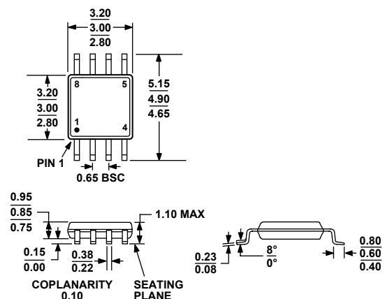
Figure 51. 8-Lead Mini Small Outline Package [MSOP]
