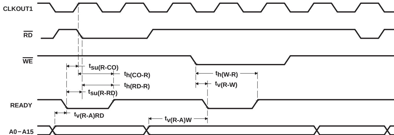
Figure 14. READY Timing
