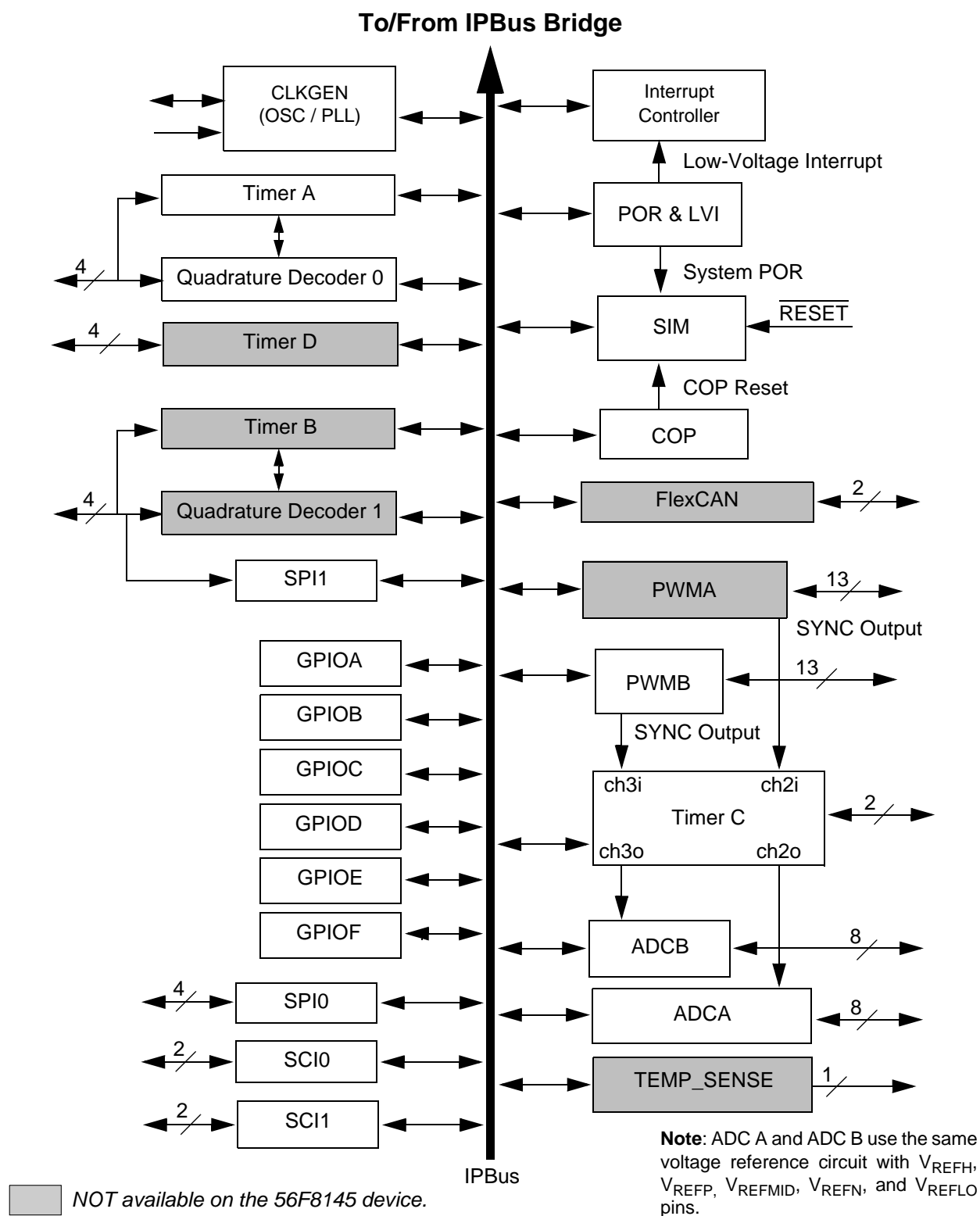
Figure 1-2 Peripheral Subsystem
