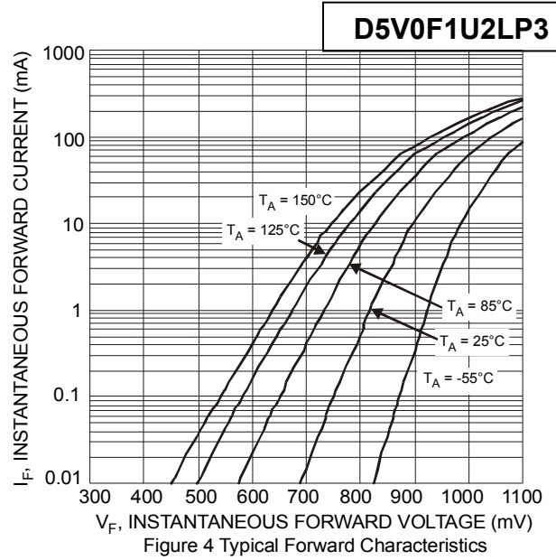
Figure 4 Typical Forward Characteristics
