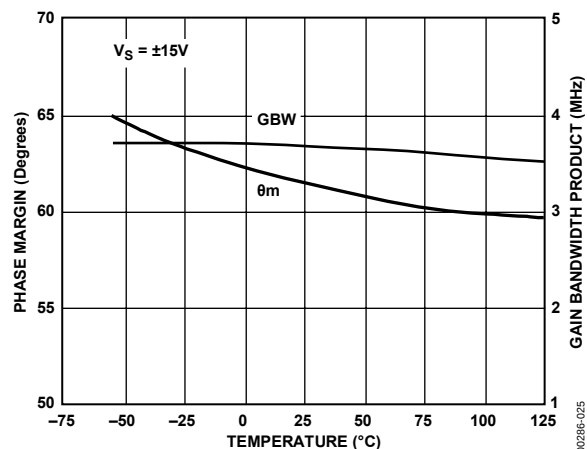
Figure 26. Gain Bandwidth Product and Phase Margin vs. Temperature @ \pm 15\text{V}
