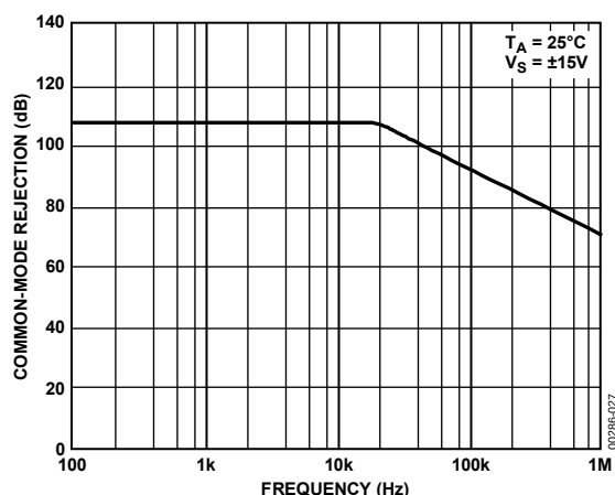
Figure 28. Common-Mode Rejection vs. Frequency @ \pm 15\text{V}
