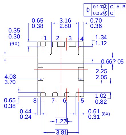
BOTTOM VIEW OPTION - A (SAWN TYPE)
