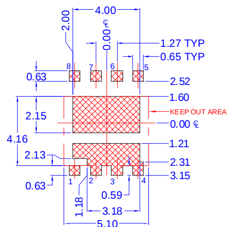
RECOMMENDED LAND PATTERN FOR SAWN / PUNCHED TYPE
