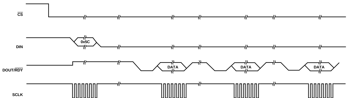
Figure 31. Continuous Read
