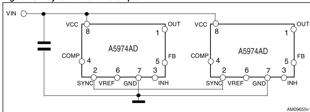
Figure 29. Synchronization example
