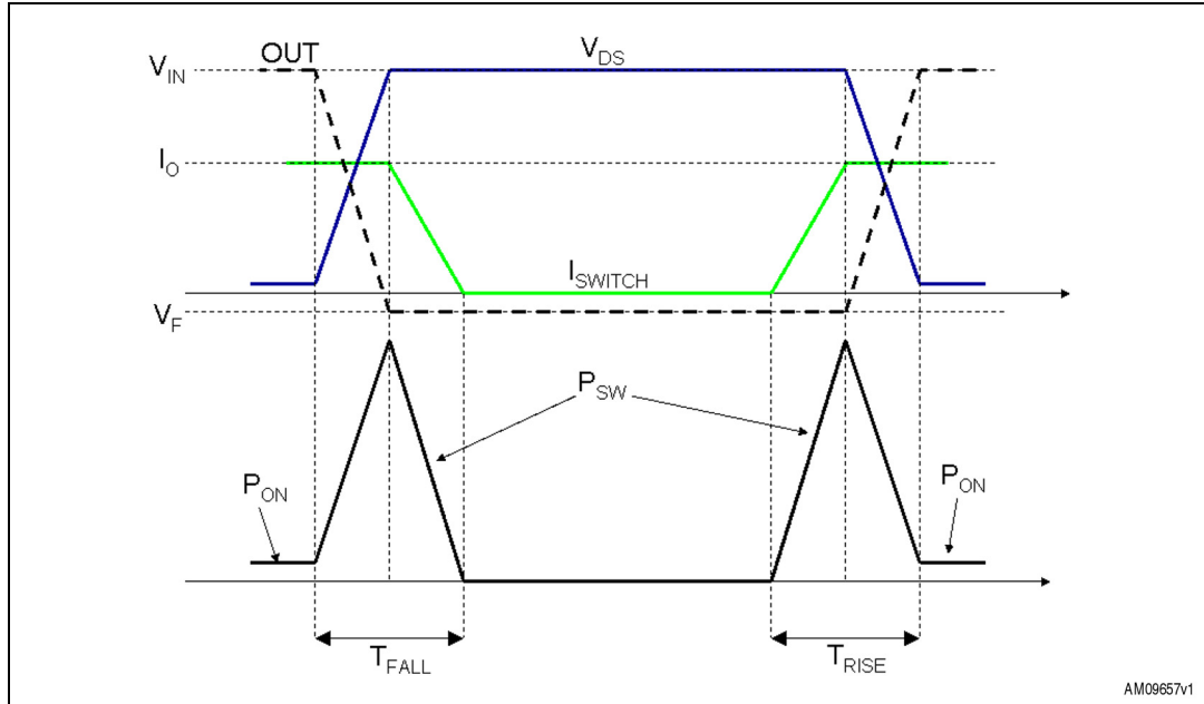
Figure 14. Switching losses
