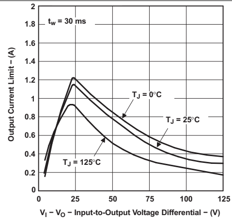
Figure 2. Output Current Limit vs Input-to-Output Voltage Differential
