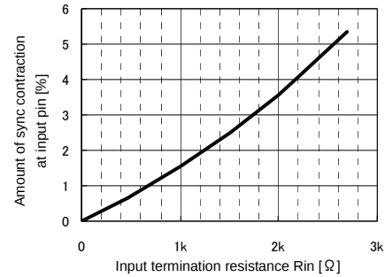
Fig. 18. Relation between Input Pin Termination Impedance and Amount of Sync Contraction
