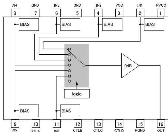
Fig.4 BH76363FV
