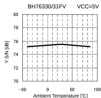
Fig.56 SN_V vs. Ambient Temperature
