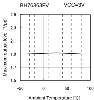
Fig.70 Vom vs. Ambient Temperature
