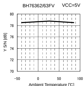
Fig.96 SN_V vs. Ambient Temperature
