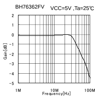
Fig.79 Frequency Response
