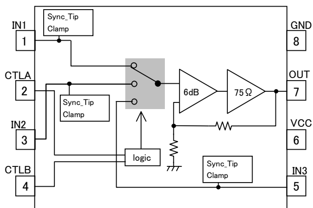
Fig.1 BH76330FV
