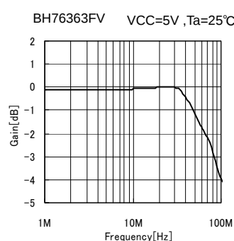
Fig.80 Frequency Response
