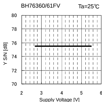
Fig.55 SN r vs. Supply Voltage
