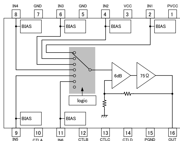
Fig.2 BH76361FV
