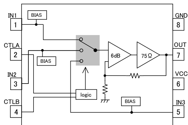
Fig.2 BH76331FV
