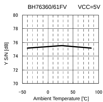
Fig.56 SN r vs. Ambient Temperature
