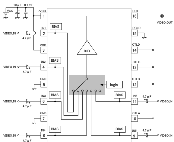
Fig.10 BH76363FV
