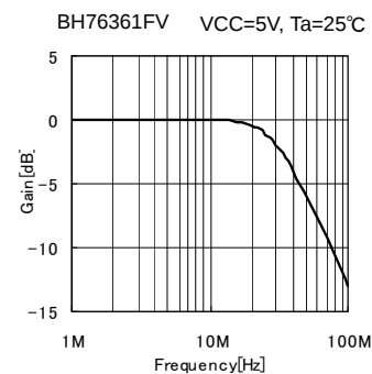
Fig. 40 Frequency Response
