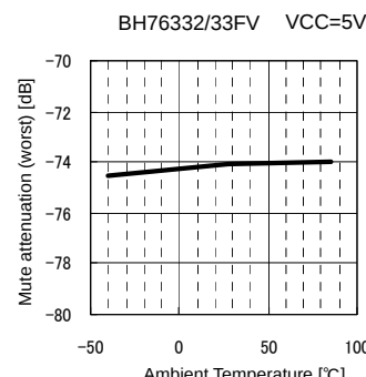
Fig.84 MT(worst) vs. Ambient Temperature
