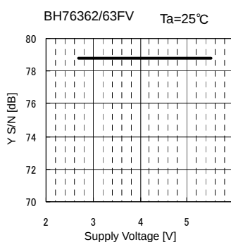
Fig.95 SN_V vs. Supply Voltage
