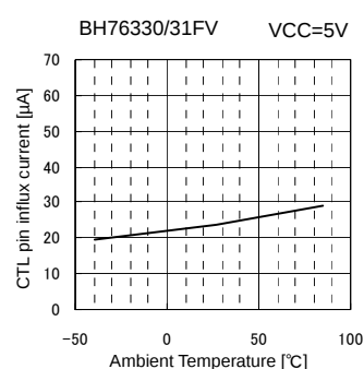
Fig.46 I_{TH} vs. Ambient Temperature (Voltage applied to CTL pin = 2V)
