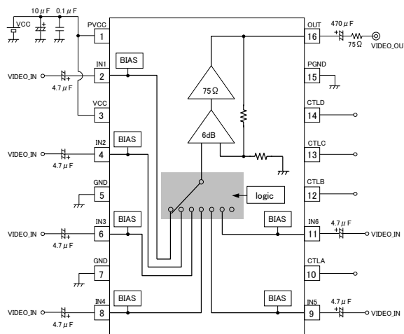
Fig.8 BH76361FV
