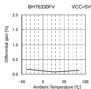
Fig.48 DG vs. Ambient Temperature
