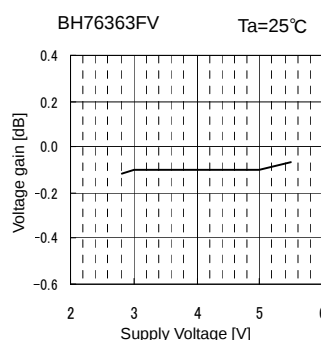
Fig.73 G v vs. Supply Voltage
