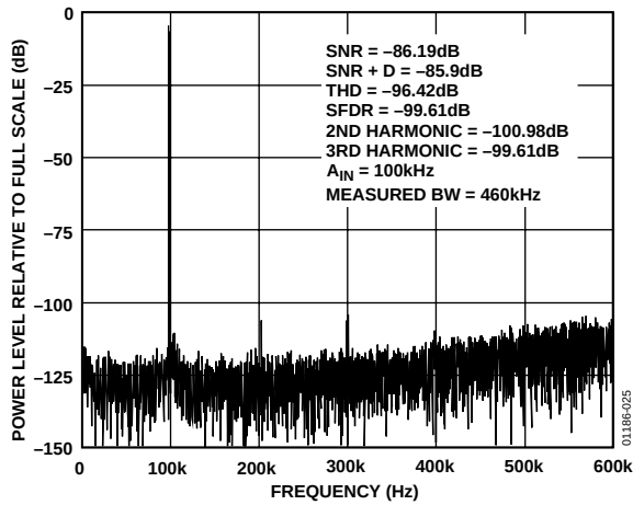
Figure 25. 16 K Point FFT (Output Data Rate = 1.2 MHz)
