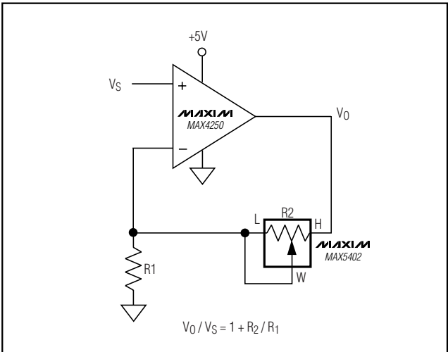
Figure 5. Noninverting Amplifier
