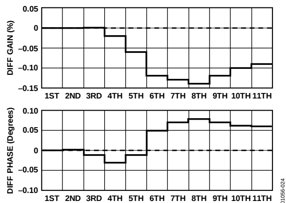
Figure 24. Differential Gain and Phase @ V_S = \pm 5V ; R_L = 1k\Omega
