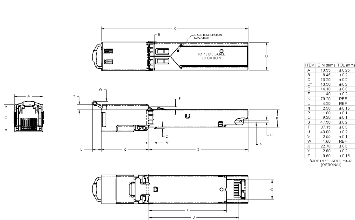
Figure 2. FCLF8520P2BTL, FCLF8521P2BTL and FCLF8522P2BTL mechanical dimensions
