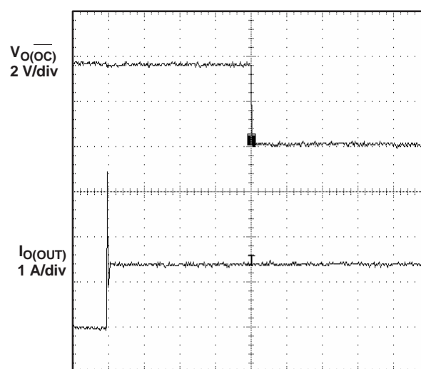
Figure 9. 1- \Omega Load Connected to Enabled Device
