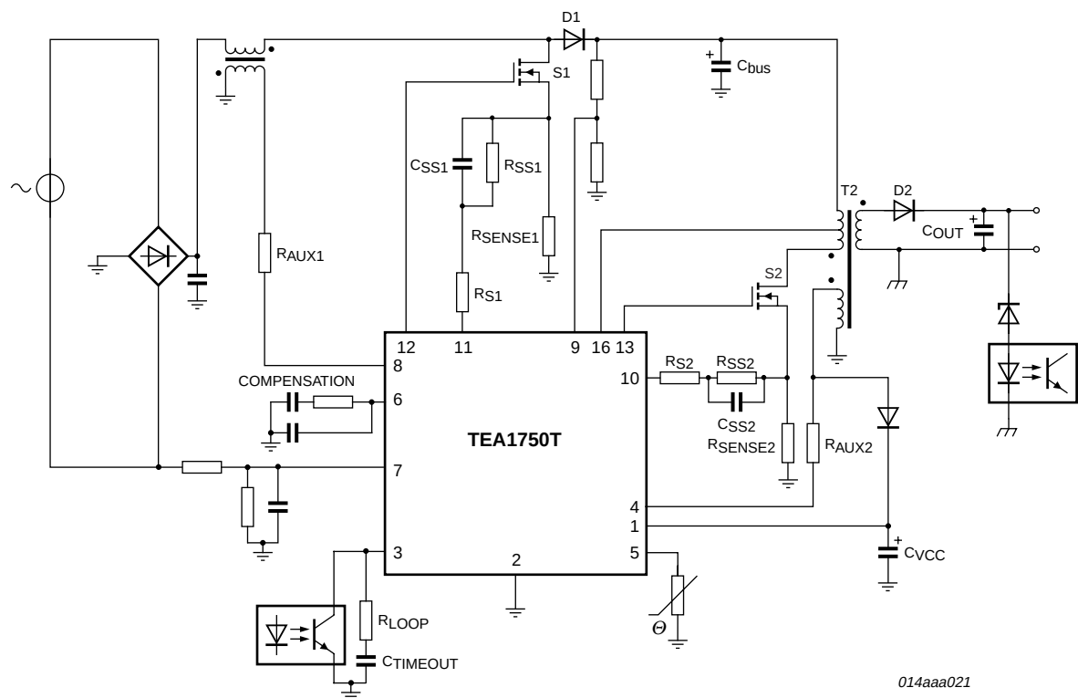
Fig 14. Typical application diagram of TEA1750
