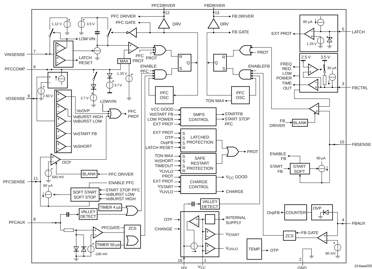
Fig 1. Block diagram
