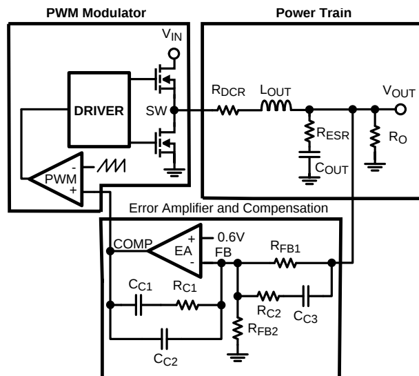
Figure 33. Loop Diagram
