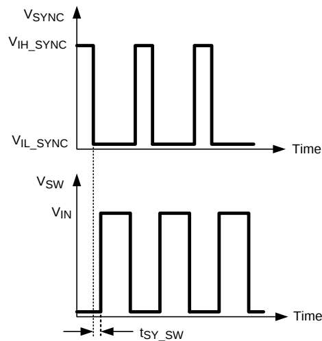
Figure 25. Frequency synchronization
