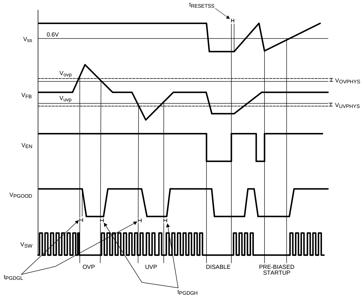
Figure 27. PGOOD Conditions
