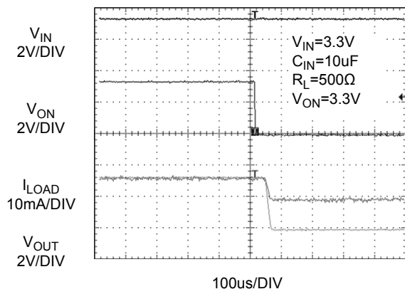
Figure 11. FPF2024 T_{OFF} Response
