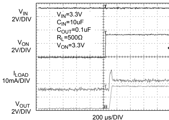
Figure 10. FPF2024 T_{ON} Response
