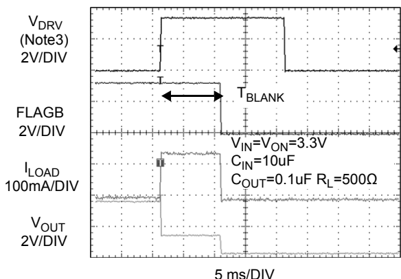
Figure 12. FPF2024 T_{BLANK} Response
