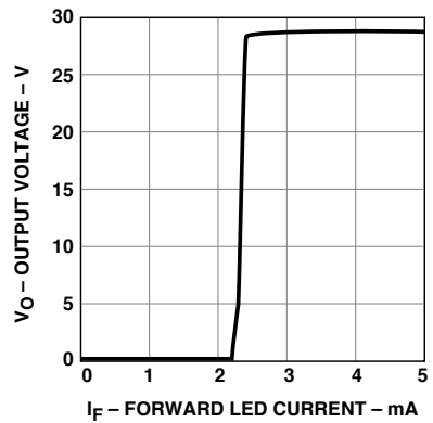
Figure 15. Transfer Characteristics.
