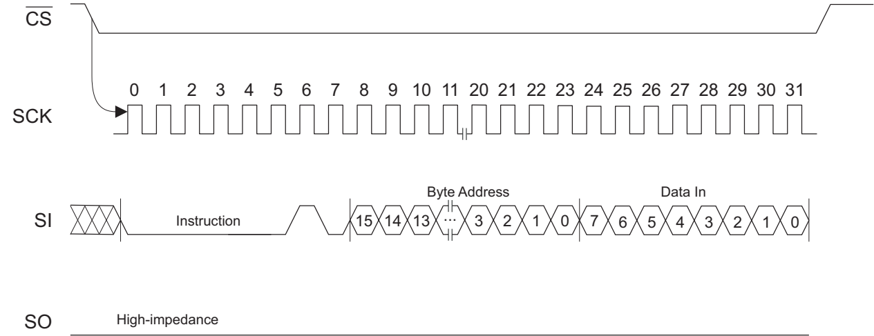
Figure 6-7. Write Timing
