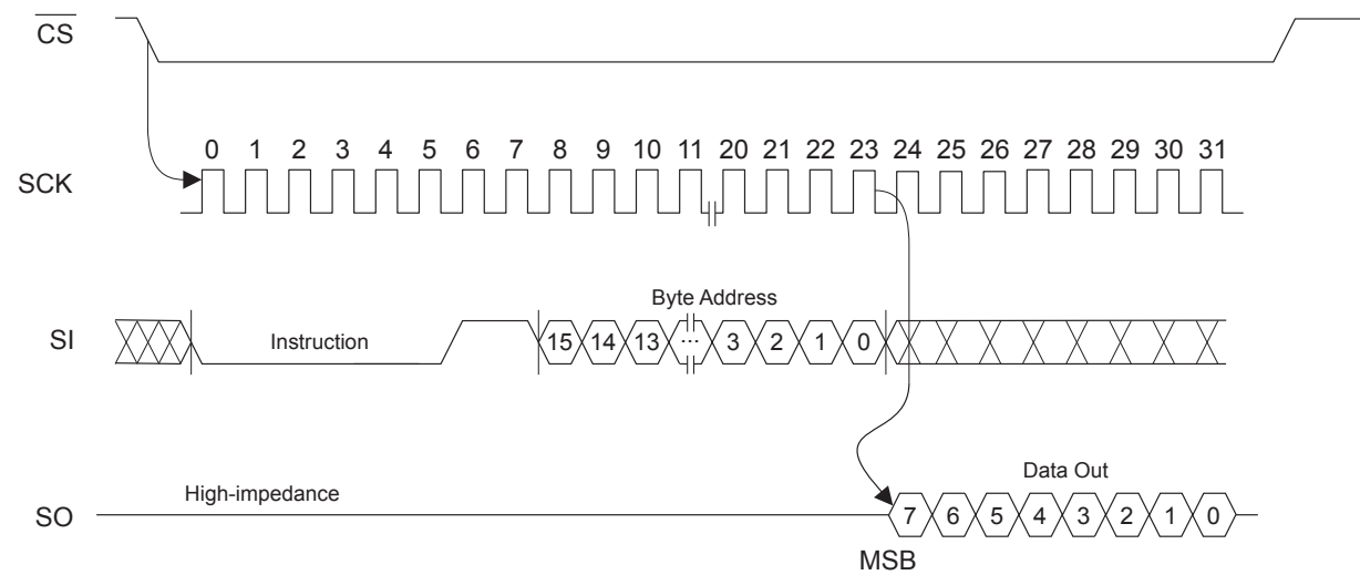
Figure 6-6. Read Timing
