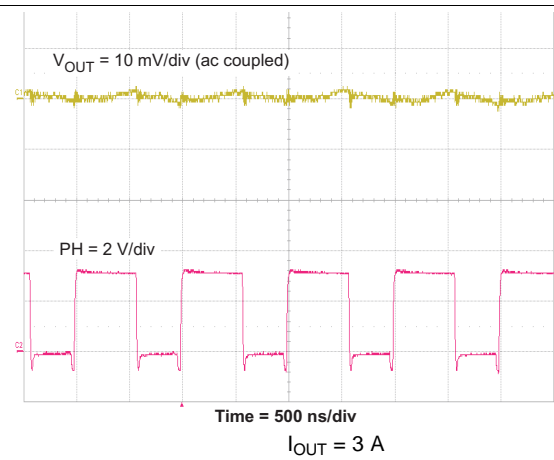
Figure 49. Input Ripple
