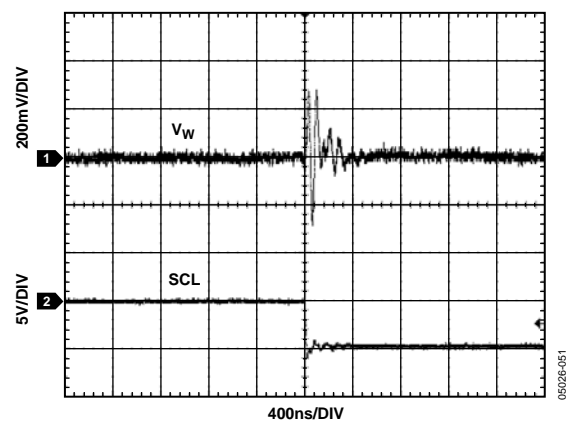
Figure 29. Digital Feedthrough
