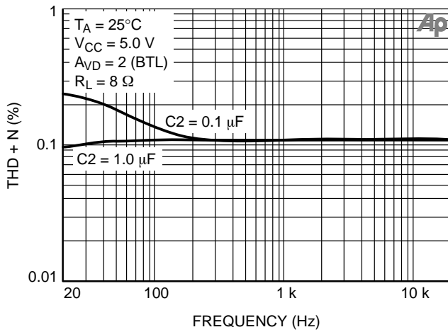
Figure 2. THD + N vs. Frequency ( P_L = 500 \text{ mW} )
