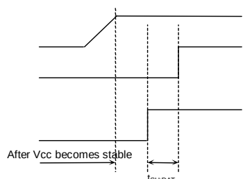
Figure 54. When SCL= 'L' and SDA= 'L'
