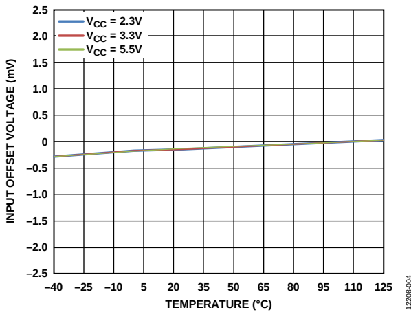
Figure 5. Input Offset Voltage ( V_{OS} ) vs. Temperature for Various Supply Voltages ( V_{CC} ), V_{CM} = 1\text{ V}
