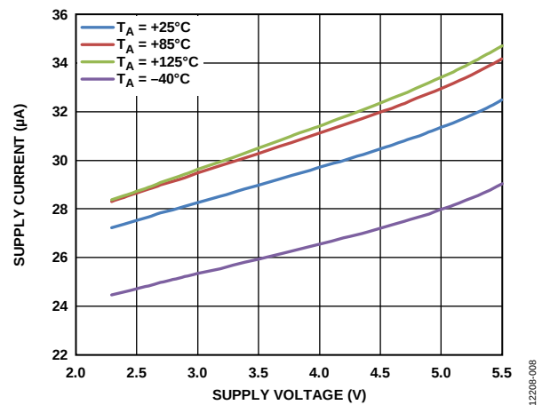
Figure 9. Supply Current vs. Supply Voltage at Output High Voltage for Various Temperatures
