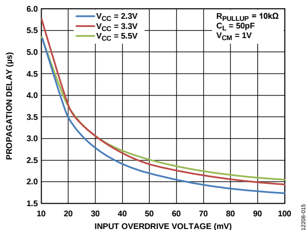
Figure 16. Propagation Delay vs. Input Overdrive Voltage, Low to High
