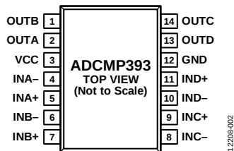
Figure 2. SOIC Pin Configuration
