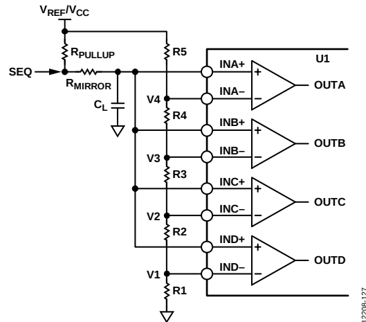
Figure 28. Circuit Configuration for a Mirrored Voltage Sequencer
