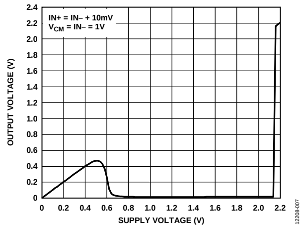
Figure 8. Output Voltage ( V_{OUT} ) vs. Supply Voltage ( V_{CC} ), R_{PULLUP} = 10\text{ k}\Omega
