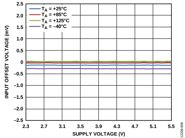
Figure 7. Input Offset Voltage ( V_{OS} ) vs. Supply Voltage ( V_{CC} ), V_{CM} = 1\text{ V} for Various Temperatures
