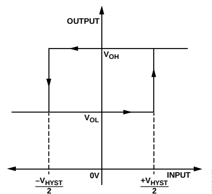
Figure 21. Comparator Hysteresis Transfer Function
