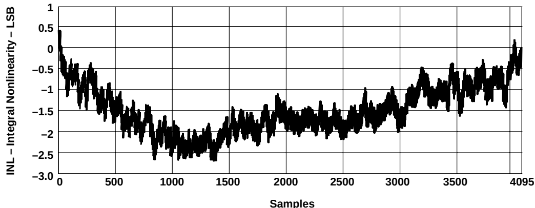
Figure 16. Integral Nonlinearity With Input Code
