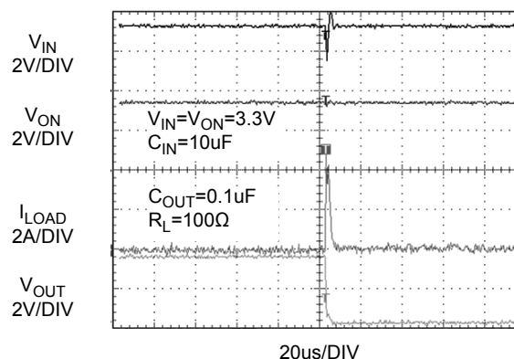
Figure 16. PPF2024 Short Circuit Response Time (Output shorted to GND while the switch is in normal operation)
