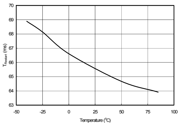
Figure 2. T_{Restart} vs. Temperature
