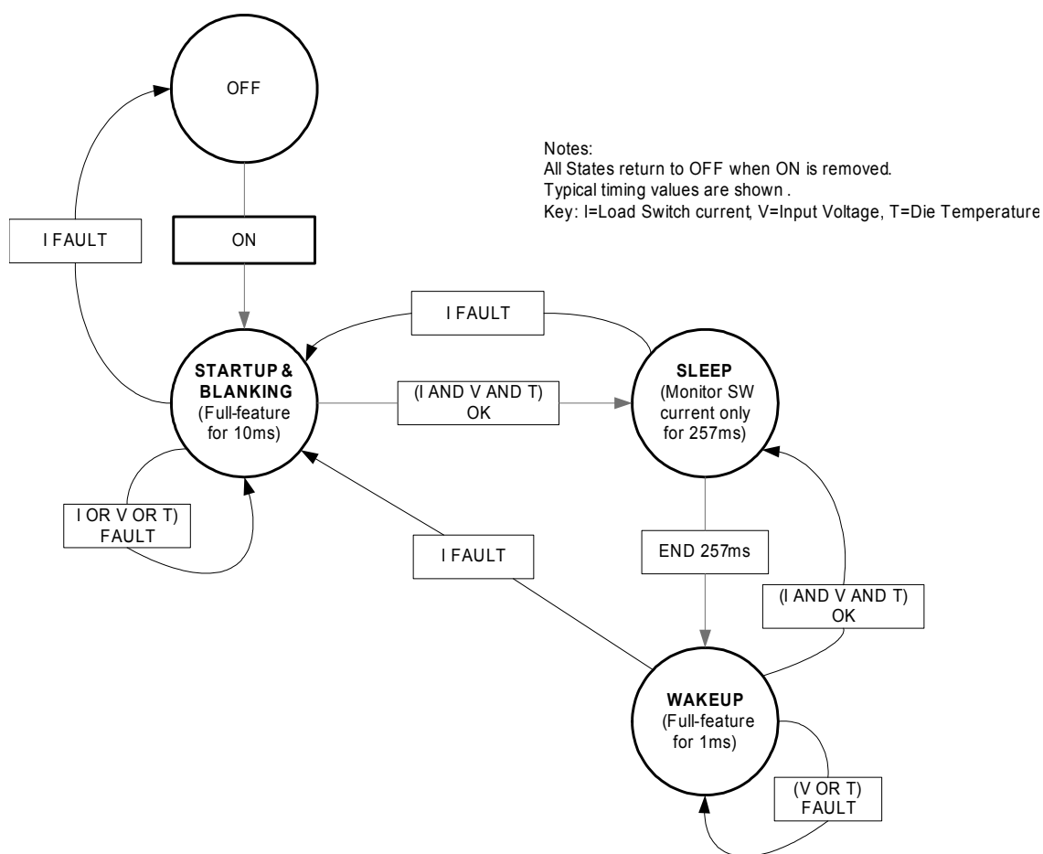
Figure 22. Representative State Diagram of FPF2026
