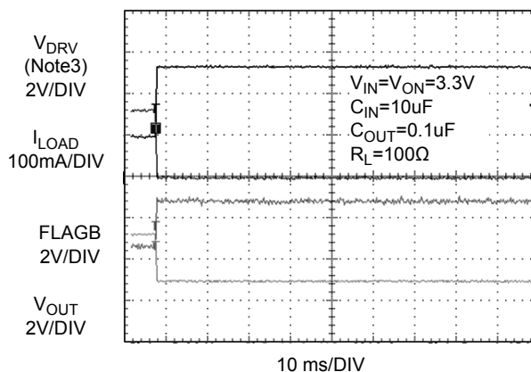
Figure 18. PPF2027 Over-Current Over-Current condition is applied while device is in normal operation (FLAGB inserts immediately and reports the fault condition)
