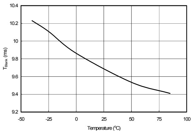
Figure 4. T_{Blank} vs. Temperature
