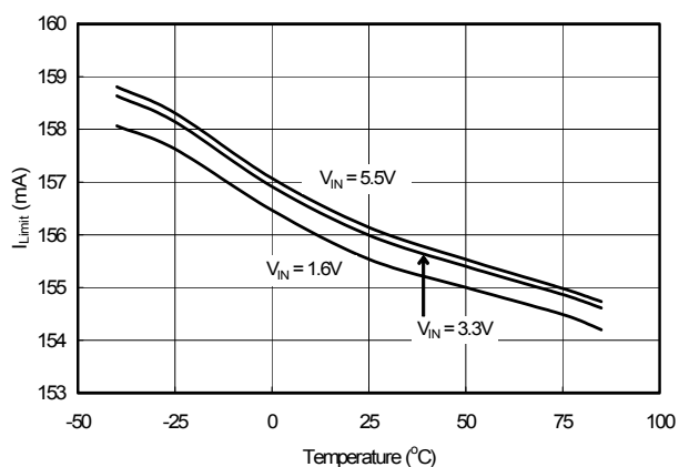
Figure 8. I_{Limit} vs. Temperature
