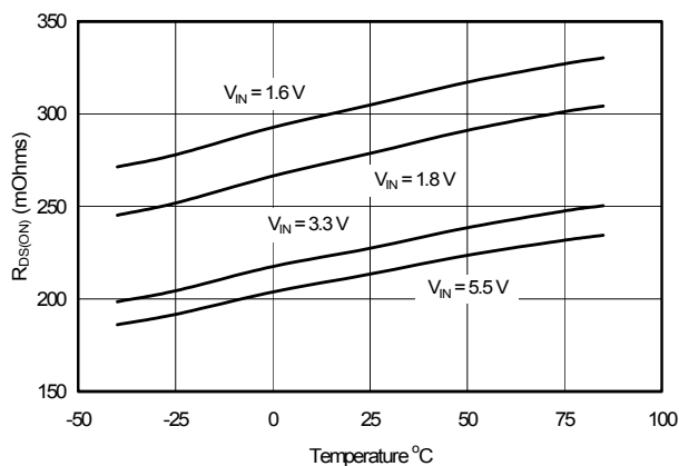
Figure 6. R_{DS(ON)} vs. Temperature
