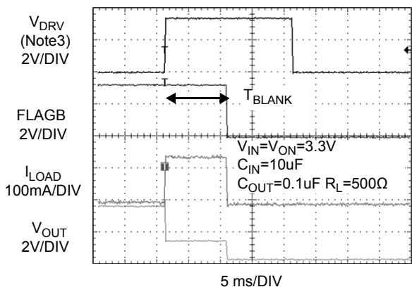
Figure 12. PFP2024 T_{BLANK} Response
