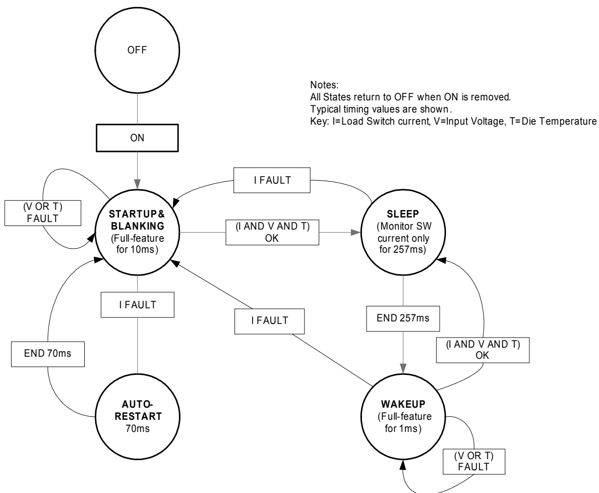
Figure 21. Representative State Diagram of FPF2024/5
