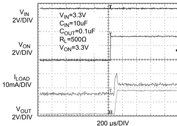
Figure 10. PFP2024 T_{ON} Response
