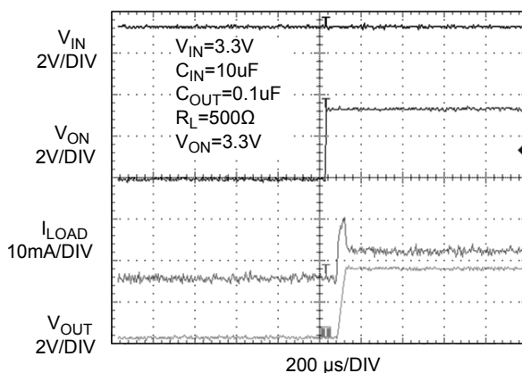
Figure 10. PPF2024 T_{ON} Response
