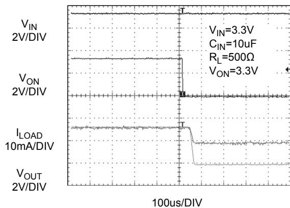
Figure 11. PPF2024 T_{OFF} Response
