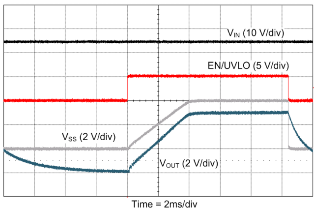
Figure 24. EN/UVLO Startup at V_{IN} = 24V and R_{LOAD} = 100\Omega
