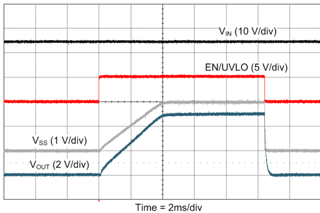
Figure 22. EN/UVLO Startup at V_{IN} = 24V and I_{OUT} = 1A
