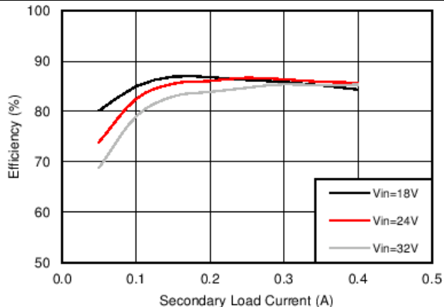
Figure 30. Efficiency vs. I_{OUT2}
