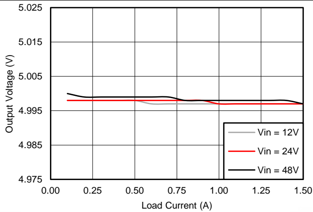
Figure 20. Load Regulation
