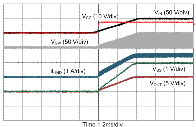
Figure 25. Startup at V_{IN} = 48V and R_{LOAD} = 10\Omega
