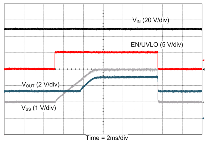
Figure 23. Pre-Bias Startup at V_{IN} = 48V and R_{LOAD} = 3\Omega
