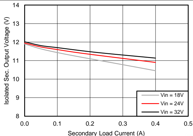
Figure 29. Load Regulation
