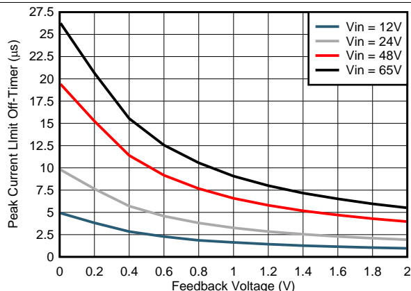
Figure 7. T_{OFF} ( I_{LIM} ) vs. V_{FB}
