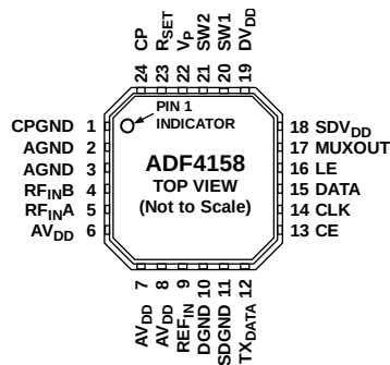
Figure 5. Pin Configuration
