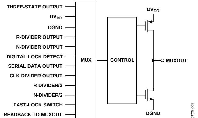
Figure 20. MUXOUT Schematic
