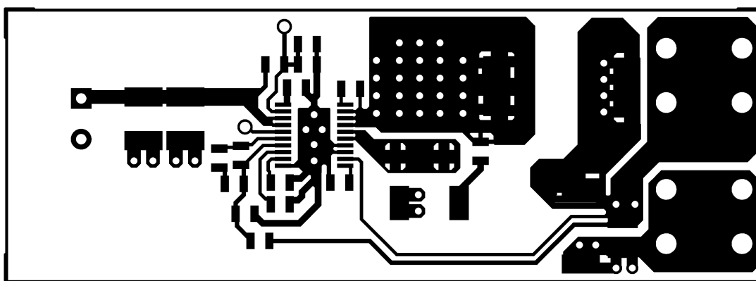
Figure 29. Component Side
