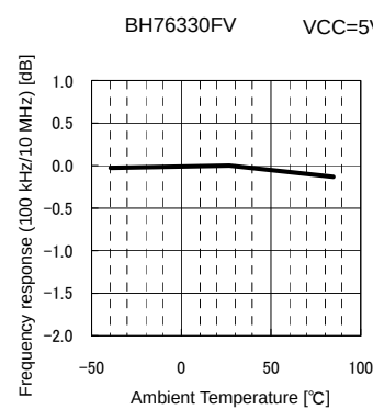
Fig. 36 G_F vs. Ambient Temperature
