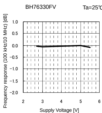
Fig. 35 G_F vs. Supply Voltage
