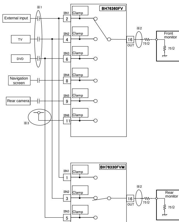
Fig. 102 Application Example in which BH76330FVM and BH76360FV Are Used Concurrently
