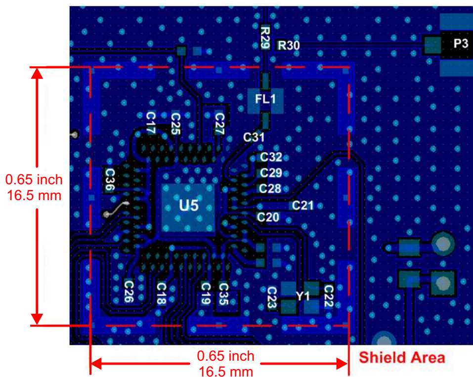
Figure 3. Component Placement
