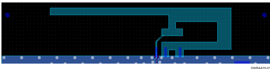
Figure 8. Inverted F Antenna on CC256x QFN Reference Design
