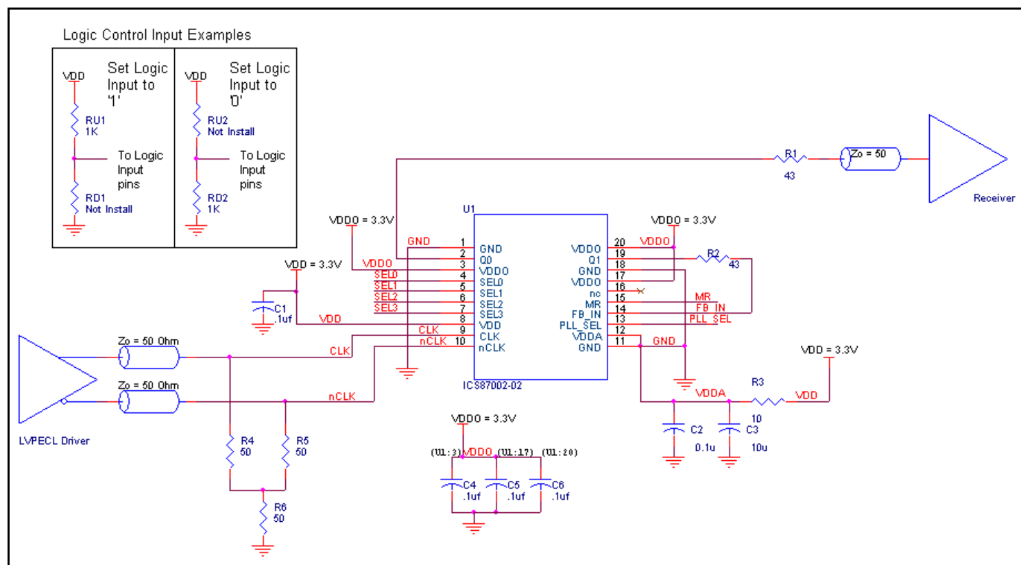
Figure 4. 87002-02 Schematic Example
