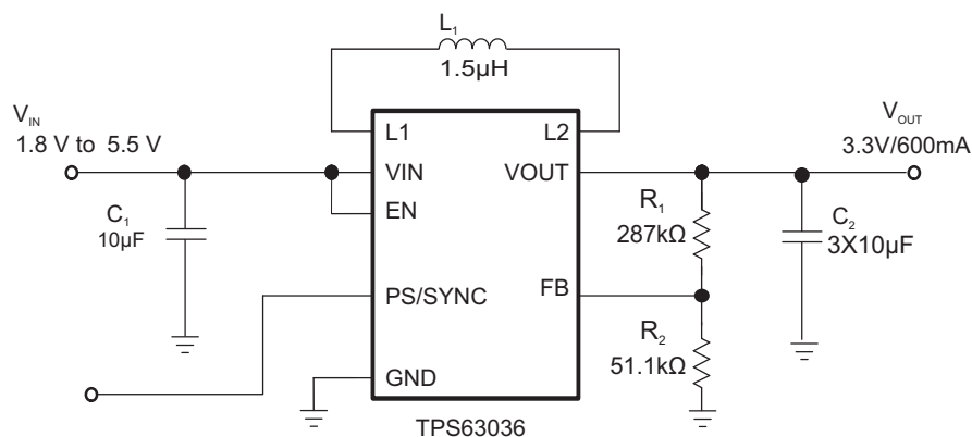
Figure 1. Typical Circuit
