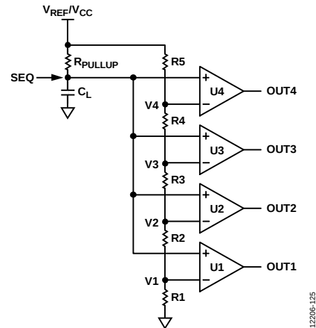
Figure 24. Programmable Sequencing Control Circuit
